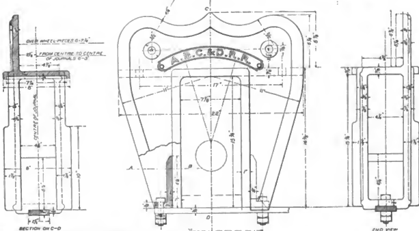
Figs. 4884-4887. Standard Pedestal for Journals. 3 1/2 in. x 7 in. Plate 14.
